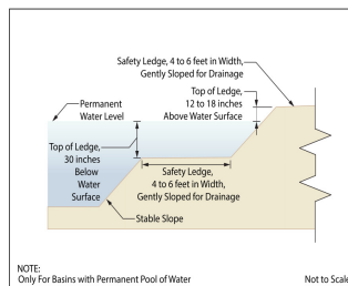
Elevation View –Basin Safety Ledge Configuration
